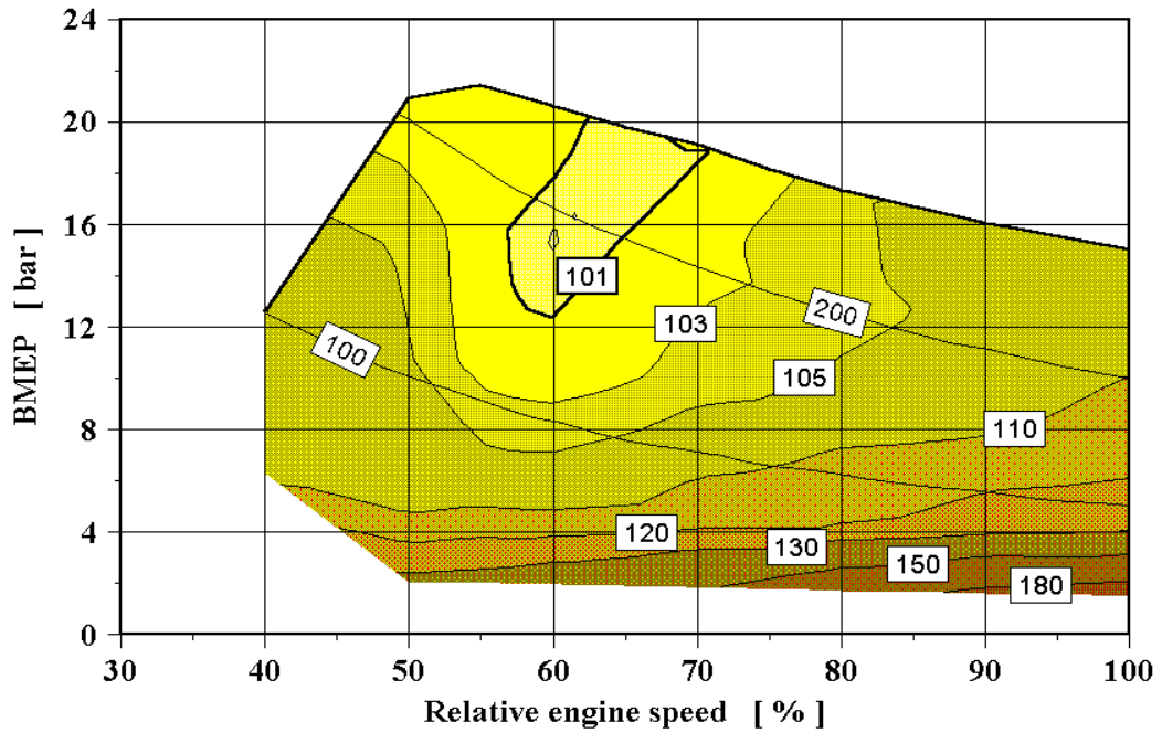
Figure 10a: b_e map with single-stage series turbocharging
